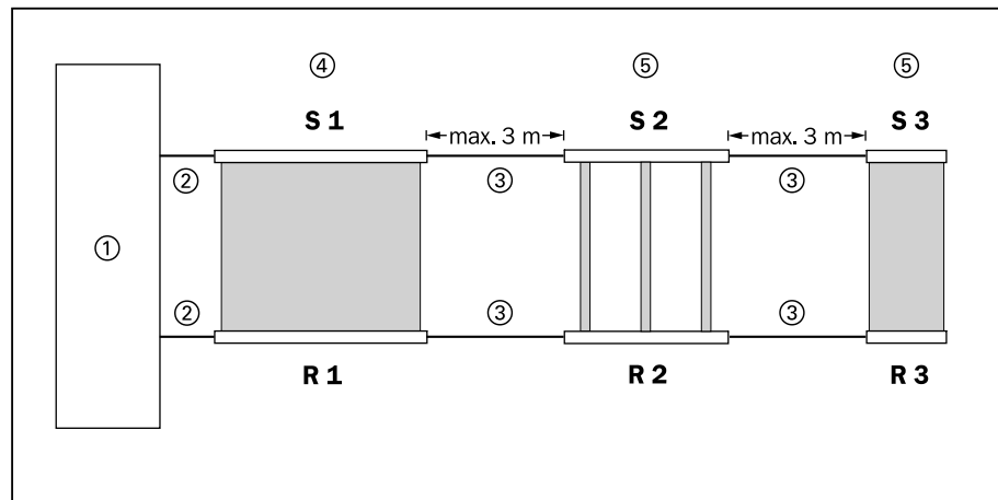
Fig. 3-7: Cascading of three devices, C 2000/M 2000
