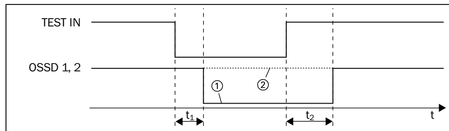
Fig. 3-11: Timing diagram of the cyclic system test in relation to switching outputs OSSD 1 and OSSD 2
