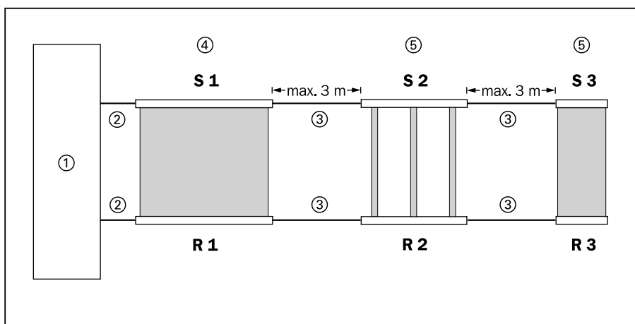
Fig. 5-15: Cable connections for cascading
