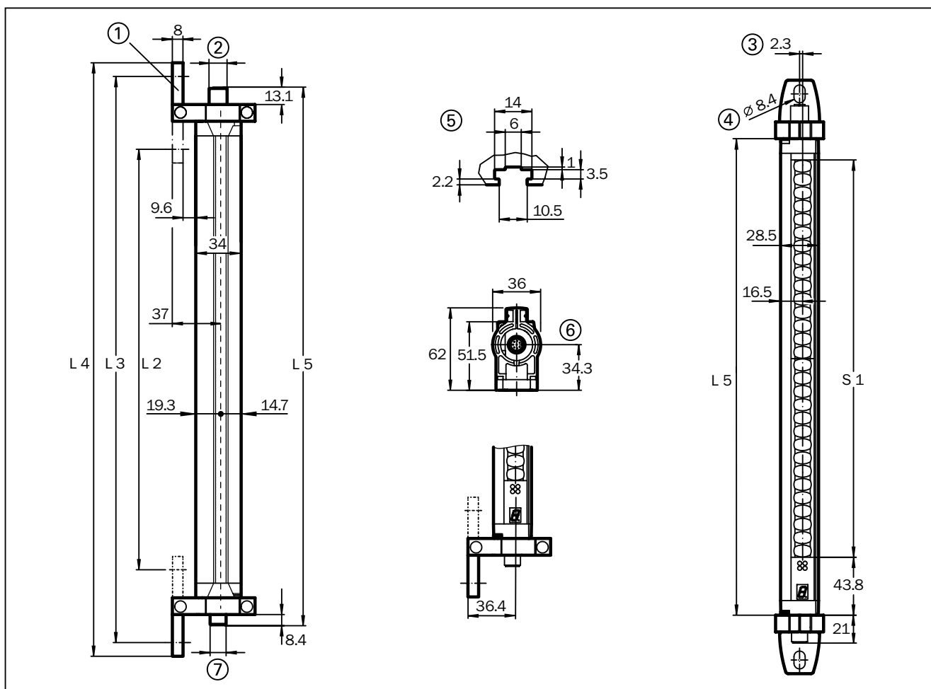
Fig. 11-3: Dimensional drawings and mechanical detail, C 2000 Cascade (sender; receiver is mirror-image), small housing, swivel mount, protective field height S_1 = 150 \dots 1200 \text{ mm}
