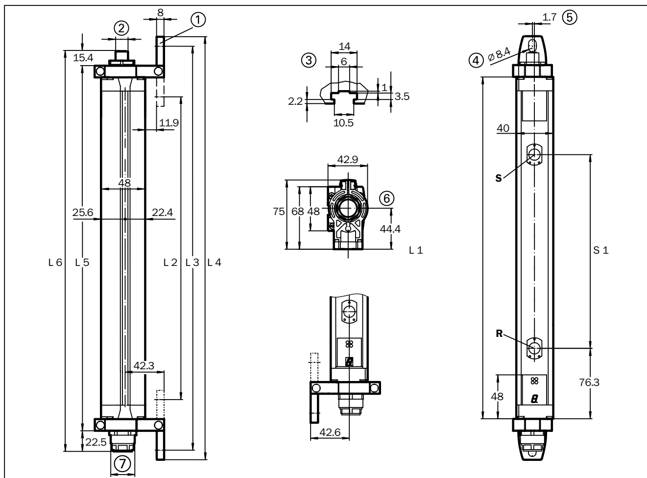
Fig. 11-8: Dimensional drawings and mechanical detail, M 2000-A/P, RES, swivel mount
