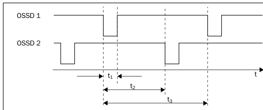
Fig. 3-15: Timing Diagram of switch outputs OSSD 1 and OSSD 2 in relation to each other
