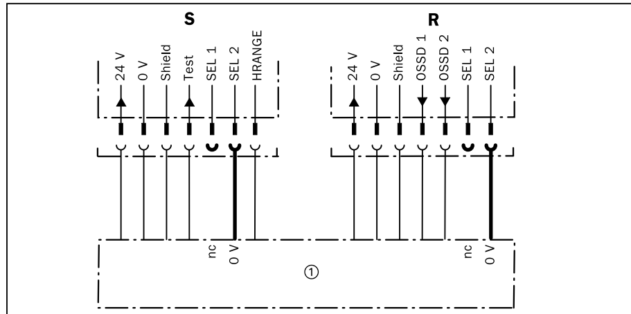
Fig. 5-10: Example: Connection of beam coding inputs for beam code 3
