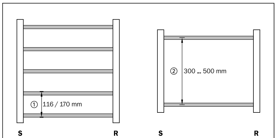
Fig. 3-2: Description, beam gap and resolution of M 2000 multi-beam photoelectric safety switch
