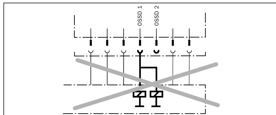
Fig. 5-8: Never interconnect OSSD outputs (= single-channel)!
