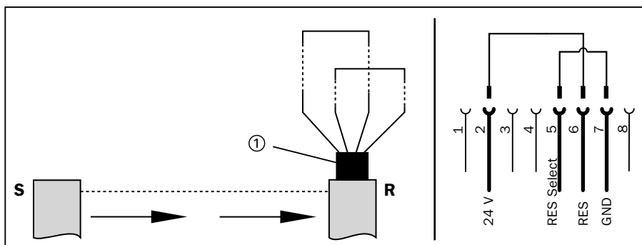
Fig. 5-14: C 2000/M 2000 with deactivated restart interlock S =Sender R =Receiver ①=Expansion socket, receiver
