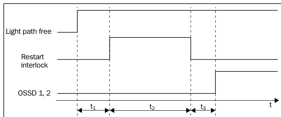
Fig. 3-13: Timing Diagram of restart interlock (RES) in relation to switching outputs OSSD 1 and OSSD 2
