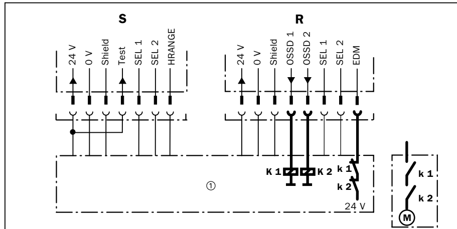
Fig. 5-12: C 2000/M 2000 with external device monitoring (EDM)
