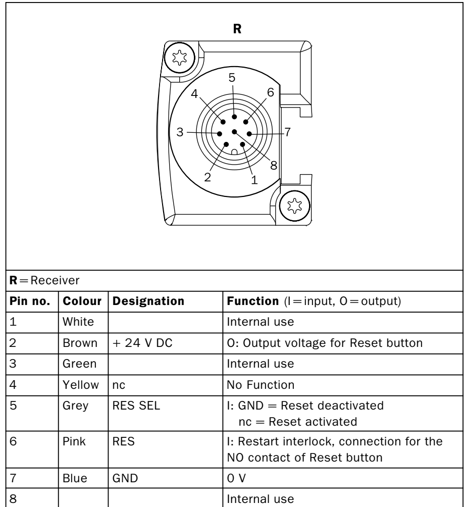
Fig. 5-6: Connection diagram of expansion socket, C 2000, M 2000 and M 2000-A/P, (RES version), nc = no connection
