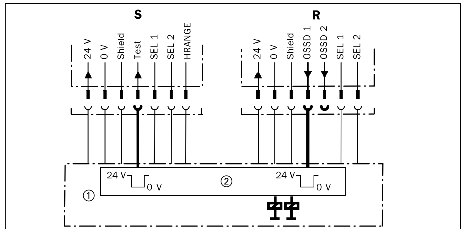
Fig. 5-9: Configuration of the cyclic system test (external test), connection of the test input and the OSSD outputs
