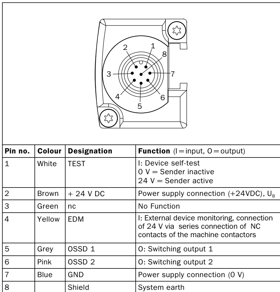
Fig. 5-5: Connection diagram, M 2000-A/P, nc = no connection
