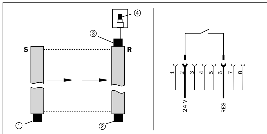
Fig. 5-13: C 2000/M 2000 with Reset button
