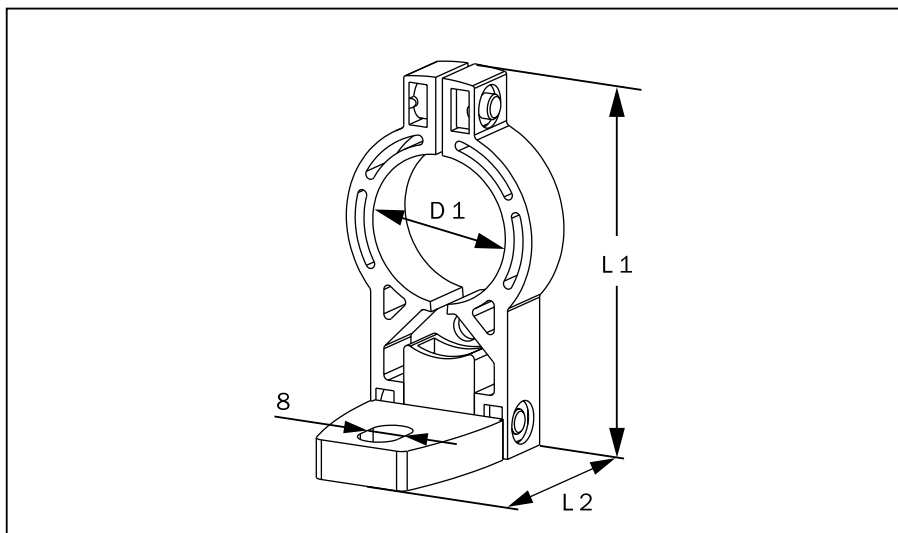
Fig. 4-2: Dimensional drawing, swivel-mount bracket for C 2000, M 2000 and M 2000-A/P
