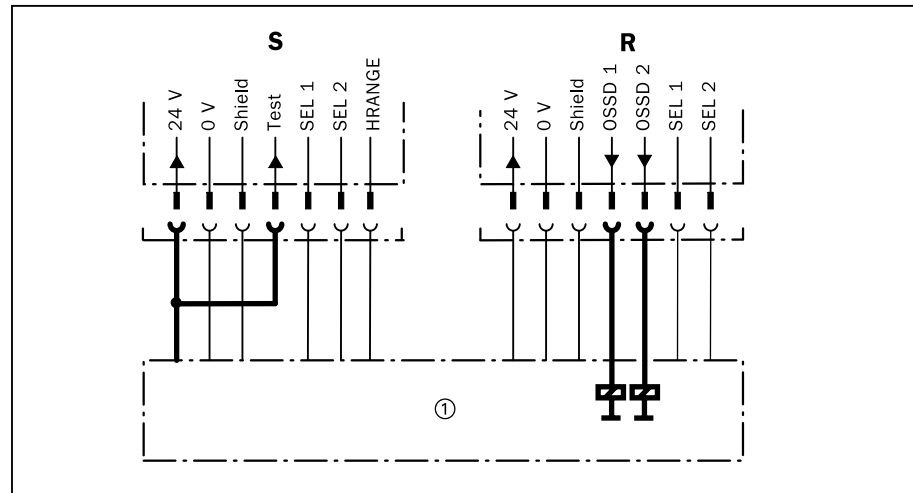
Fig. 5-7: Connection of OSSD outputs for device self-test
