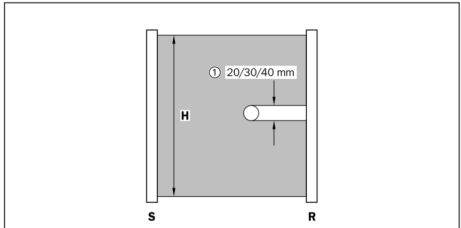
Fig. 3-1: Description and resolution, C 2000 safety light curtain
