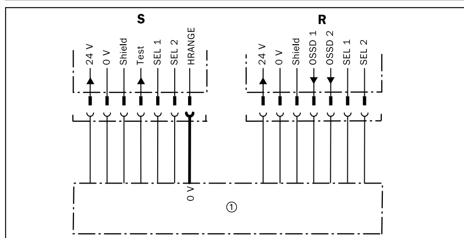
Fig. 5-11: Configuration of sender operating range, 0 V = Operating range 0 ... 6 m S = Sender R = Receiver ① = Machine control
